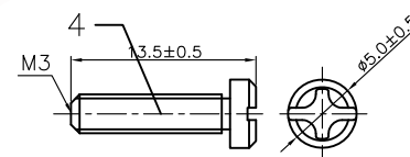
LONG SCREW
