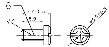
SHORT SCREW
