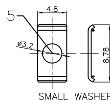
SMALL WASHER
