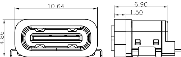
Schematic diagram with waterproof ring
