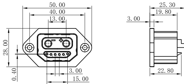
Installation size
