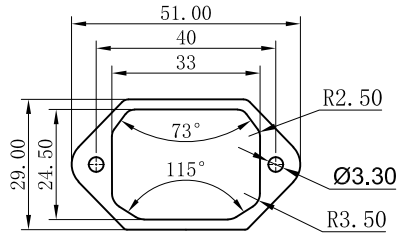
Installation size
